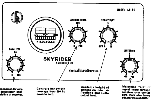
Figure 5. Skyrider Panoramic Model SP-44, view showing adjustment controls.
