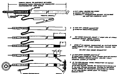
Figure 3. View Showing Cable Preparation for Permanent Installation.
